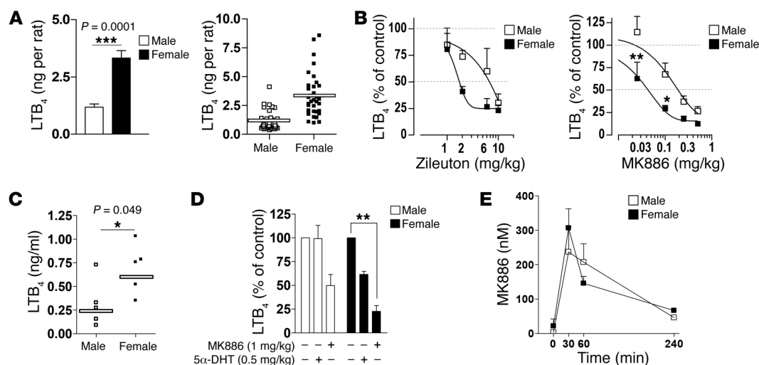
Figure 1. Sex differences in the production of LTB_4 and in the potency of LT biosynthesis inhibitors in vivo. (A) LTB_4 levels in the thoracic cavity 2 hours after \lambda -carrageenan injection in male and female rats. n = 35 (5 rats/sex in 7 experiments); unpaired 2-tailed t test. Data passed normality test. *** P < 0.001 . (B) Effects of zileuton and MK886 on pleural LTB_4 levels in male and female rats 2 hours after \lambda -carrageenan injection. Vehicle or compounds were injected i.p. 30 minutes prior to \lambda -carrageenan. Data show percentage of controls, mean + SEM. For 10 mg/kg zileuton and 0.5 mg/kg MK886, n = 10 (5 rats/sex in 2 experiments); for the other doses, n = 5 (5 rats/sex in 1 experiment). The different doses were tested in independent experiments performed side by side with male/female rats and controls. * P < 0.05 ; ** P < 0.01 vs. corresponding males, ANOVA plus Bonferroni. (C) LTB_4 levels in the peritoneal cavity 15 minutes after i.p. zymosan injection in male and female mice. n = 5 (5 mice/sex in 1 experiment); unpaired 2-tailed t test. (D) Mice received 1 mg/kg MK886 or 0.5 mg/kg 5 \alpha -DHT 30 minutes prior to zymosan injection. LTB_4 levels in the peritoneal cavity of male and female mice were assessed 15 minutes after i.p. zymosan. n = 5 (5 mice/sex in 1 experiment); ANOVA plus Bonferroni. (E) Plasma levels of MK886 after i.p. injection of 1 mg/kg in male and female mice at 0, 30, 60, and 240 minutes after administration. n = 3 (3 mice/sex in 1 experiment); no significant differences, ANOVA plus Bonferroni.
